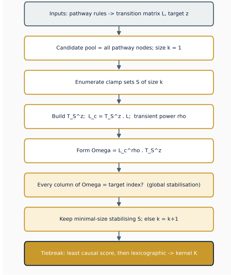
Figure 2: The forward-stabilisation kernel test. For each candidate clamp set S , the controlled operator \Omega = L_c^\rho T_S^z is formed. The set is accepted only if every column of \Omega is the target index, that is, the clamp drives every block state to target, not only the patient’s. Minimal accepted sets are kept and ties are broken deterministically. On the nine-node switch block this test is tractable; on the full 141-node network it is not.
